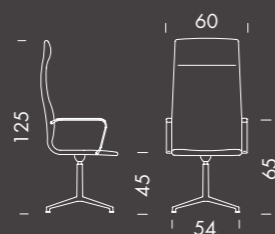
464 Swivelling
